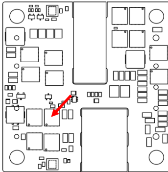
Figure 16. Temperature Monitoring Location
