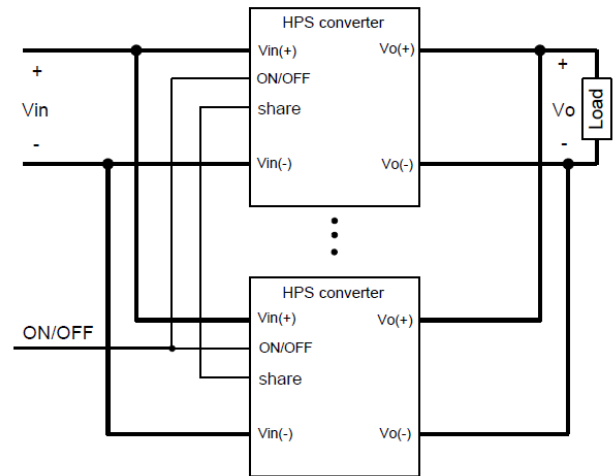
Figure 15. Circuit Configuration for Active Current Share
