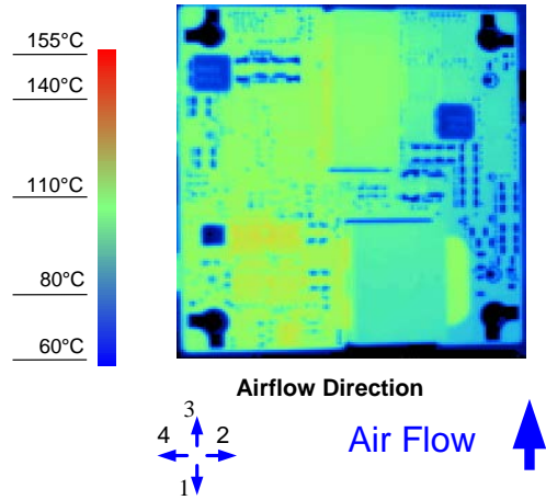
Figure 8. Thermal Image for Airflow Direction 3 (4.5A output, 55°C ambient, 200 LFM, typical Vin, open frame, unit soldered onto a fixture board)
