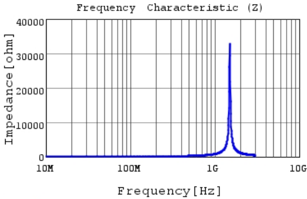
LQG15WZ75NG02 |Z|
