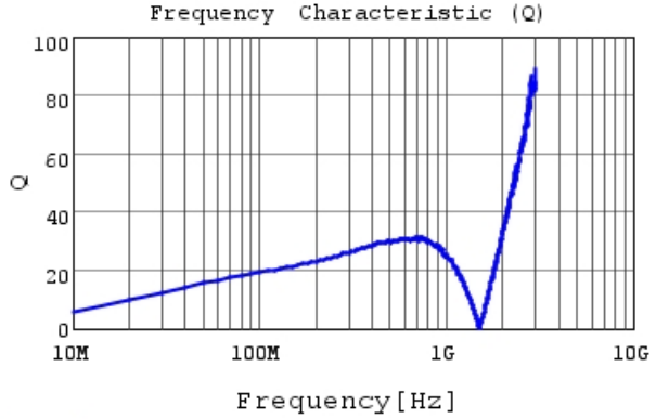
LQG15WZ75NG02 Q
