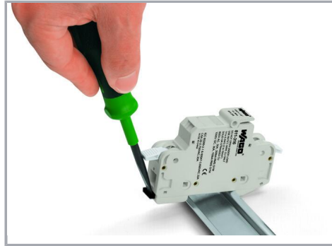
Removing a terminal block from the DIN-rail.
