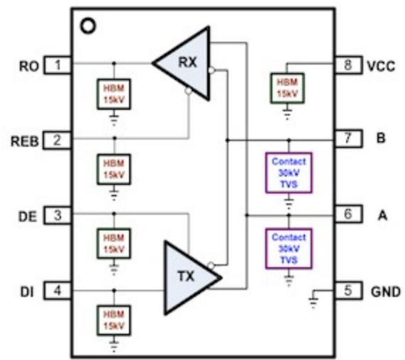
Functional Block of AZRS3082
