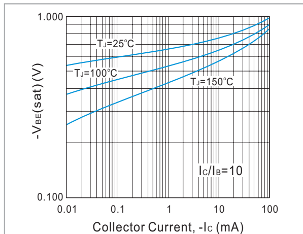
Fig. 4. Typical V_{BE(sat)} vs Collector Current
