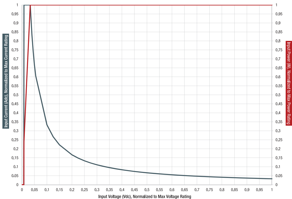
ALx Series MagnaLOAD Normalized Operating Profile - 1000 Vdc Models
