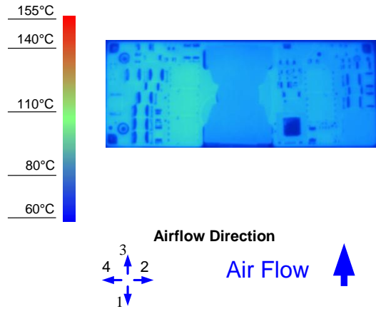
Figure 8. Thermal Image for Airflow Direction 3 (17A output, 55°C ambient, 200 LFM, typical Vin, open frame, socket interface)
