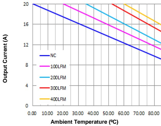
Figure 7. Current Derating Curve for Airflow Direction 3 (Ref. Fig. 8 for Airflow Direction; Vin = 36V, open frame)
