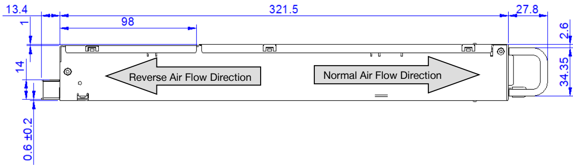
Figure 41. Side View 1
