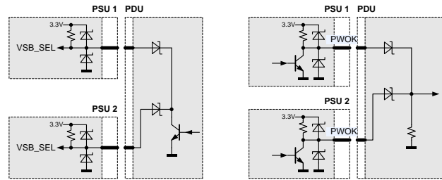
Figure 23. Interconnection of Signal Pins
