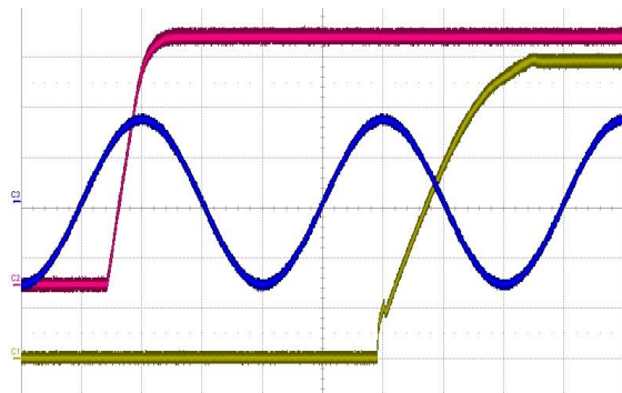
Figure 7. Turn-On AC Line 230VAC, full load (5ms/div) CH1: V_1 (2V/div) CH2: V_{\text{SB}} (1V/div) CH3: V_{\text{in}} (200V/div)
