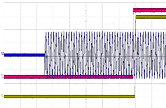
Figure 6. Turn-On AC Line 230VAC, full load (200ms/div) CH1: V_1 (2V/div) CH2: V_{\text{SB}} (1V/div) CH3: V_{\text{in}} (200V/div)
