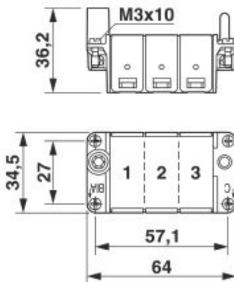
Dimensional drawing
