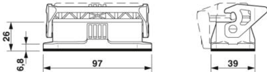
Dimensional drawing
