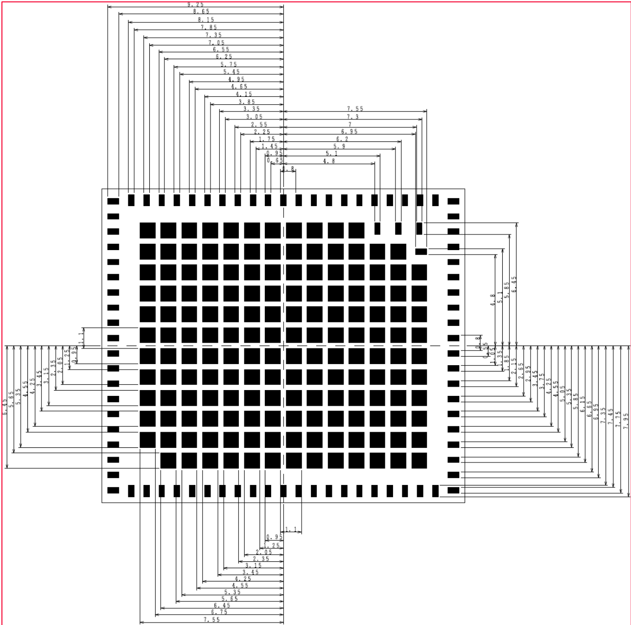
Figure 17: Land Patterns (Unit: mm)
