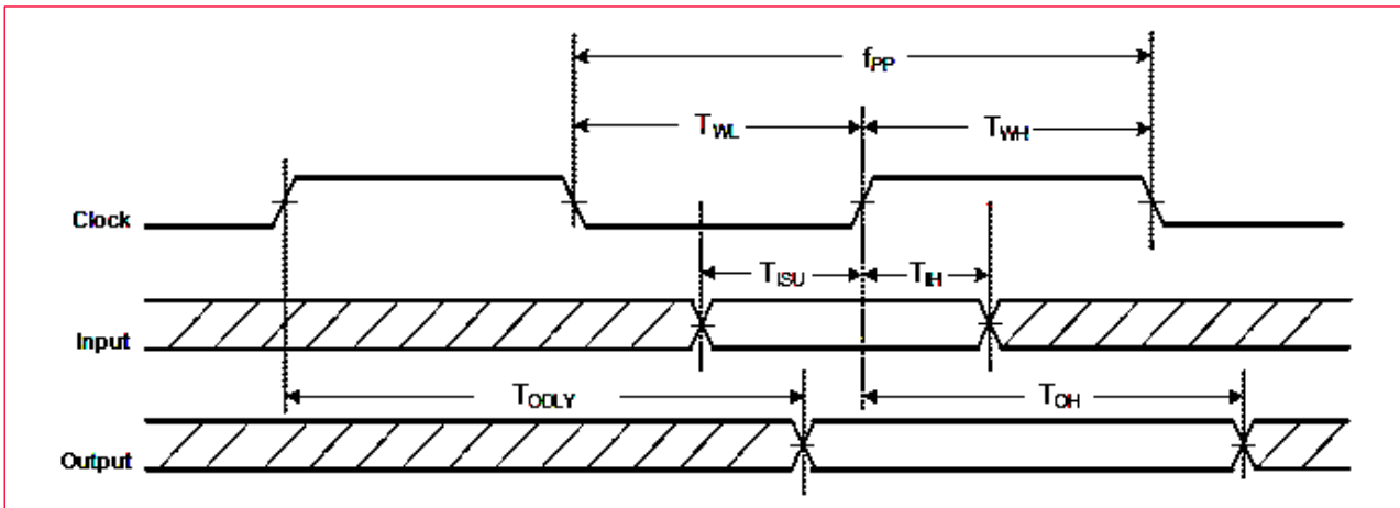
Figure 11: SDIO Protocol Timing Diagram - High Speed Mode (3.3V)
