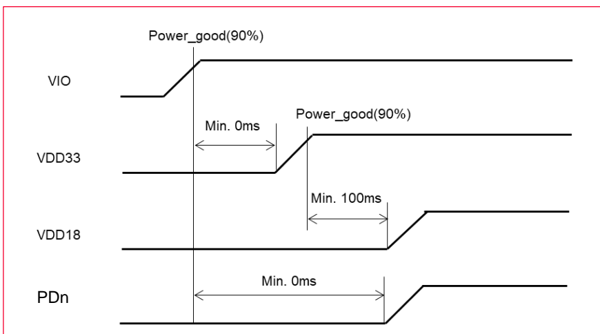
Figure 7: Power-On Sequence Graph for VIO 3.3V
