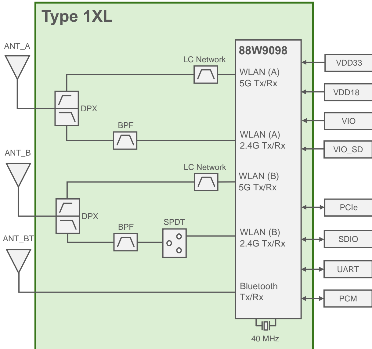
Figure 1: Block Diagram
