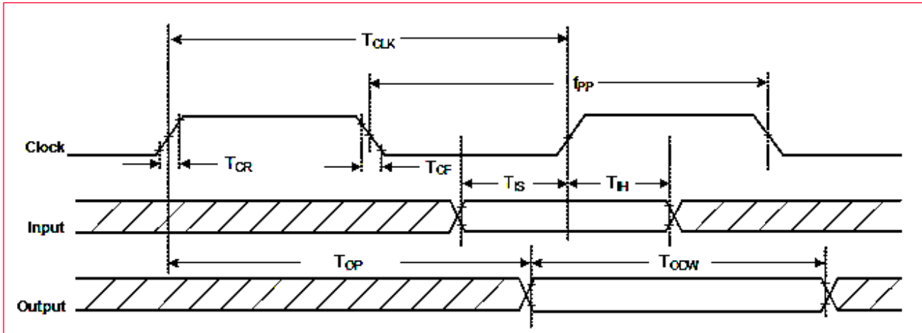
Figure 13: SDIO Protocol Timing Diagram - SDR104 Mode
