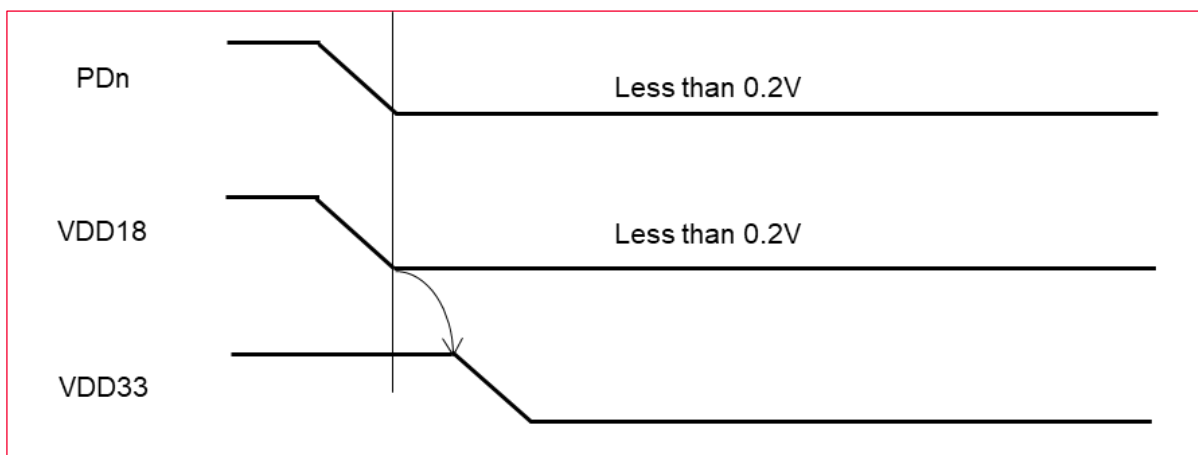
Figure 9: Power-Off Sequence Graph
