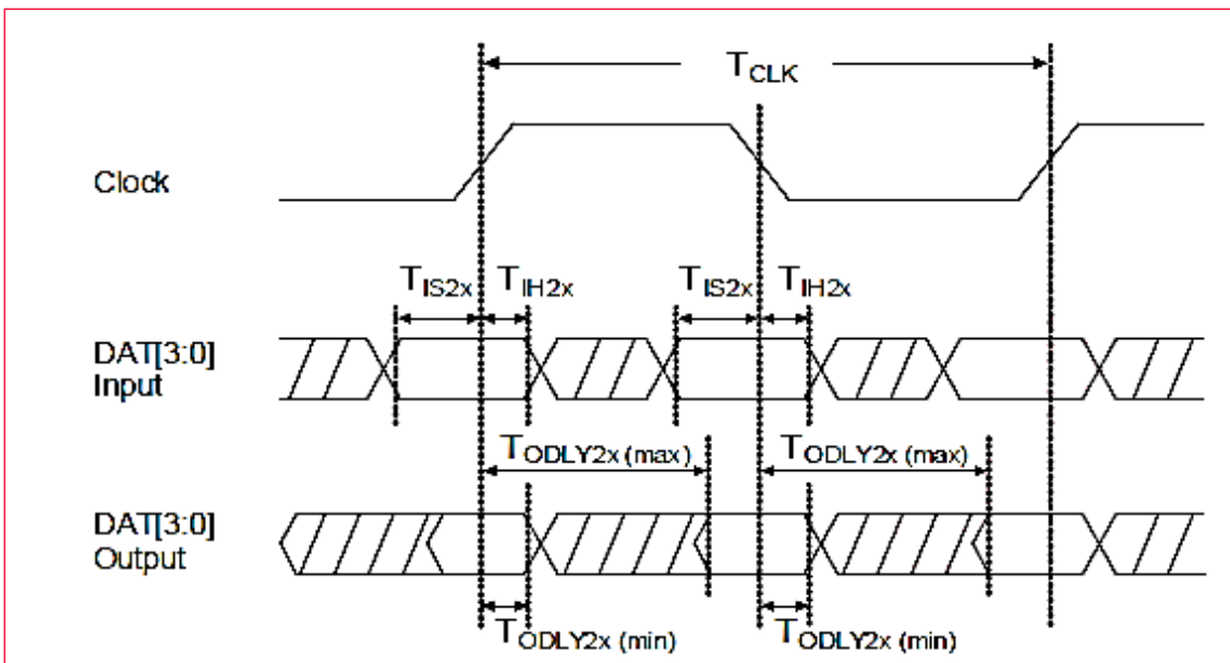
Figure 15: SDIO DAT[3:0] Timing Diagram - DDR50 Mode
