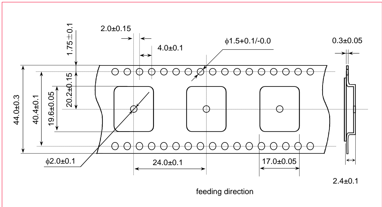
Figure 18: Dimensions of Tape (Plastic Tape)
