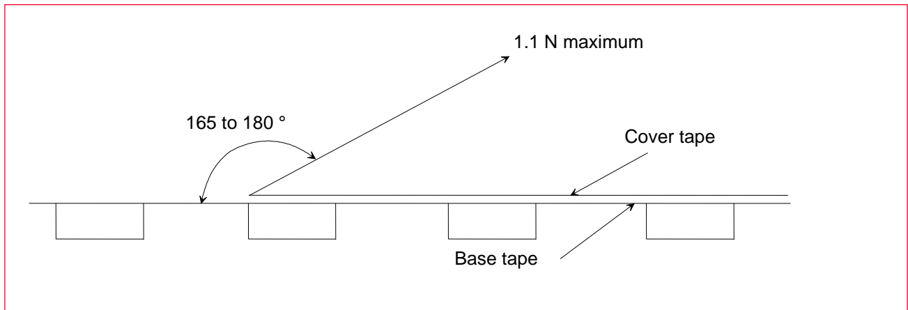
Figure 22: Peeling Force
