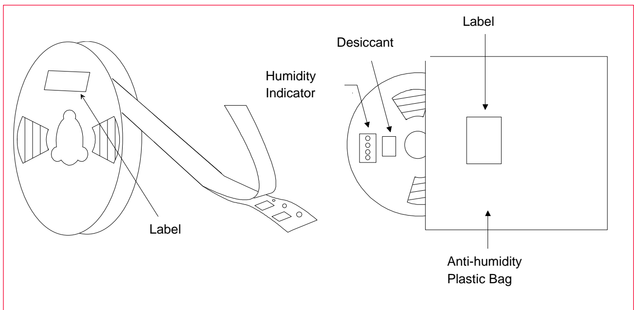
Figure 23: Humidity Proof Packing
