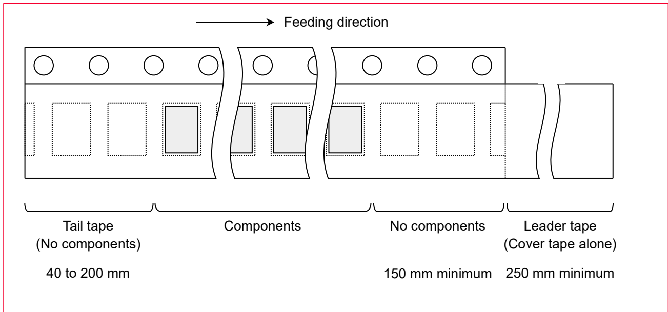
Figure 21: Leader and Tail Tape
