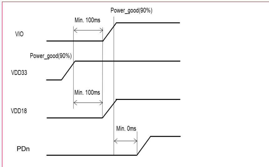
Figure 8: Power-On Sequence Graph for VIO 1.8V
