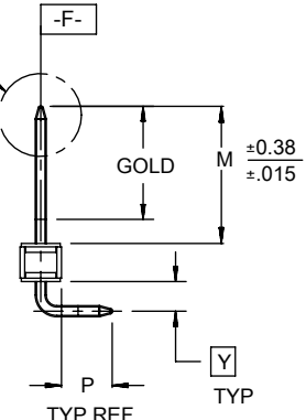
OPTIONAL KINK PIN SEE NOTE 7
