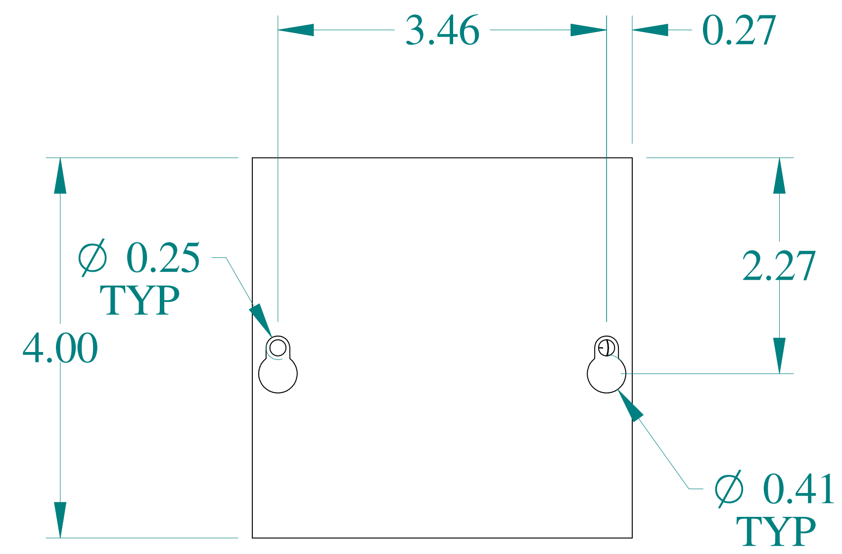
TOP VIEW
