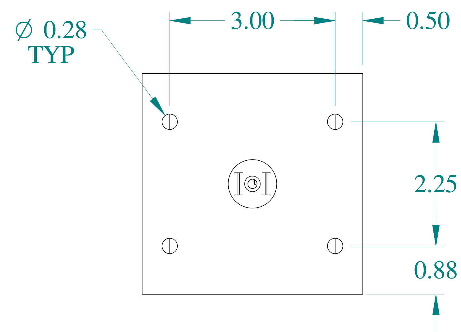
BOTTOM VIEW
