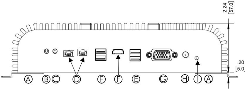
REAR VIEW
