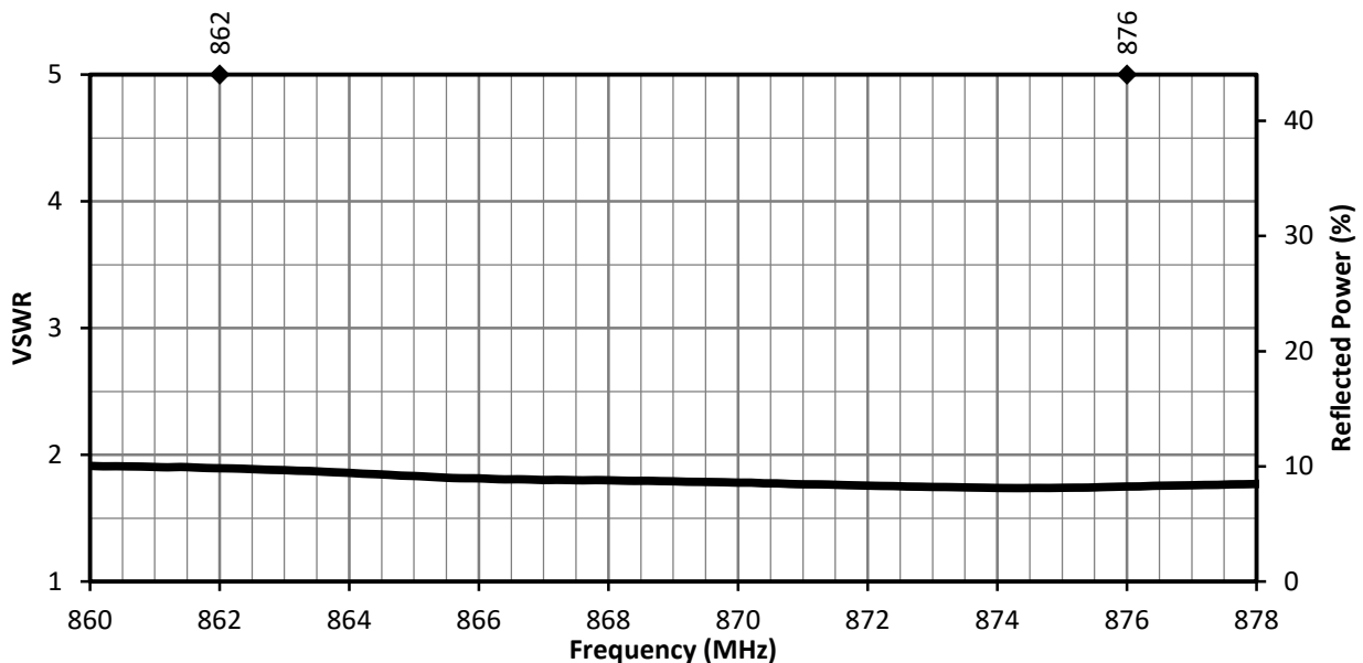
Figure 1. ANT-868-CW-RCL-SMA VSWR
