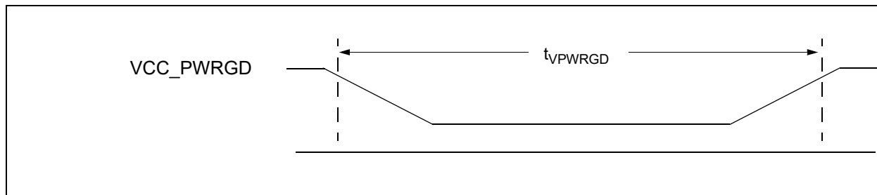
FIGURE 53-4: VCC_PWRGD TIMING
