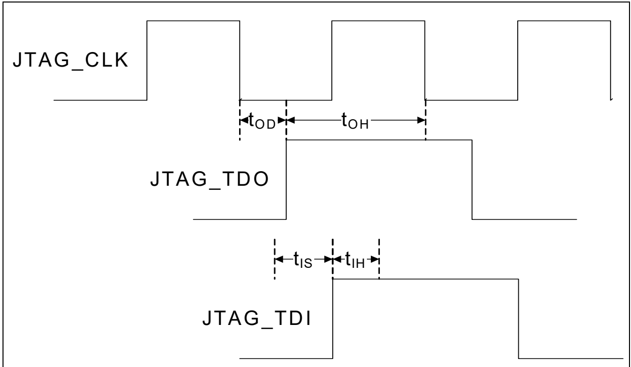
FIGURE 53-29: JTAG SETUP & HOLD PARAMETERS
