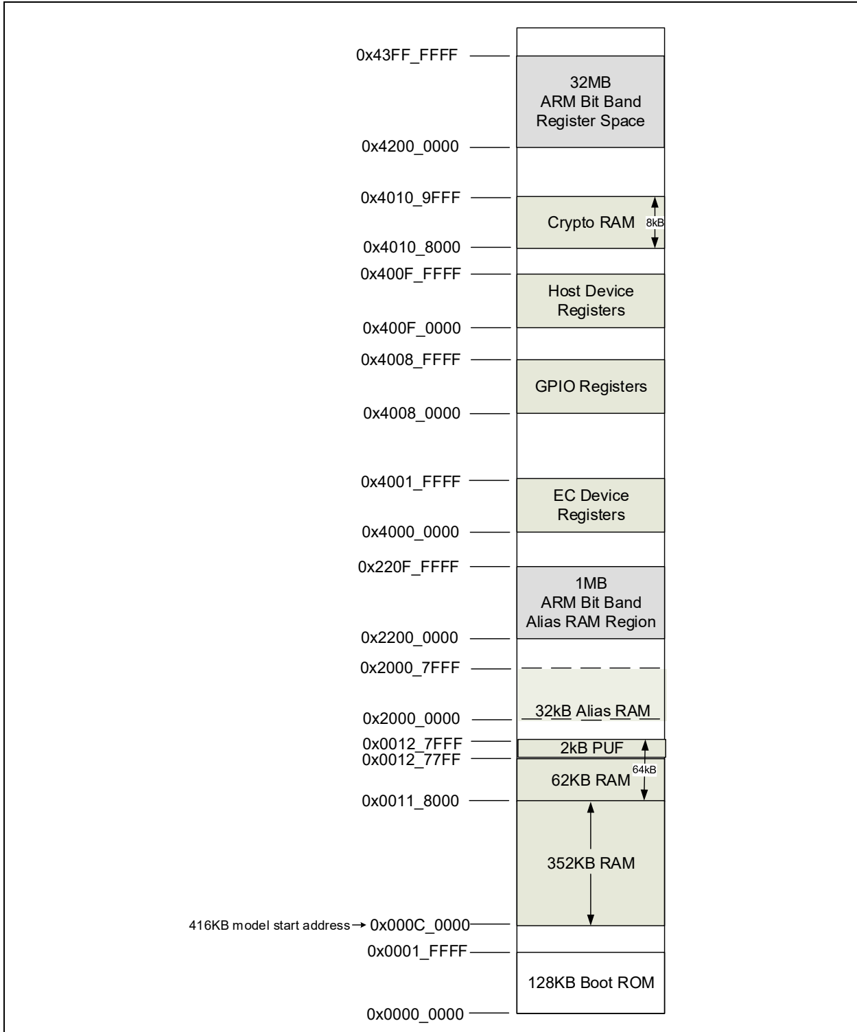
FIGURE 6-1: MEMORY LAYOUT
