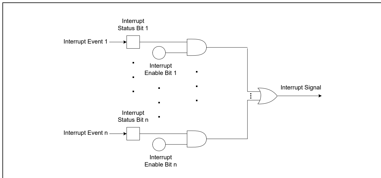
FIGURE 37-9: INTERRUPT FLOW
