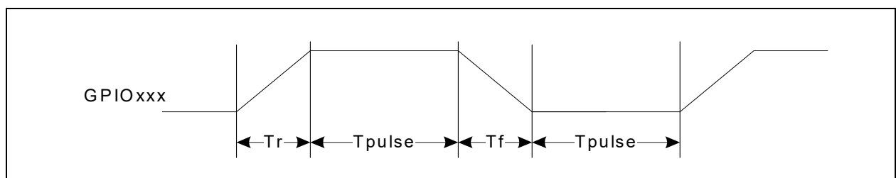
FIGURE 53-7: GPIO TIMING
