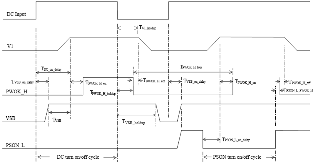
Figure 14. Timing Requirement
