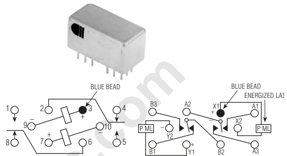
TERMINAL VIEW
