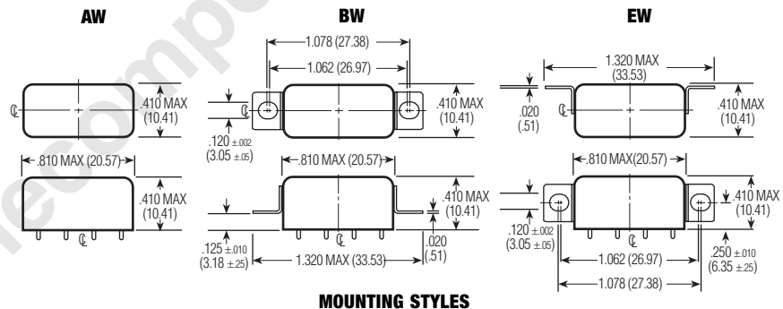
MOUNTING STYLES
