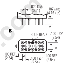
LR TERMINALS
