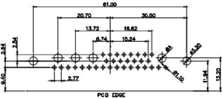
36W4 Male
