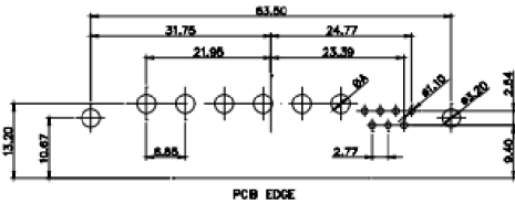
17W5 Male
