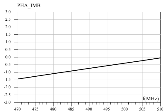
Figure 4. Phase imbalance (°)
