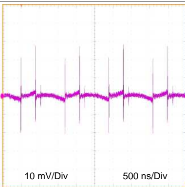
12\text{ V}_{IN} 3.3\text{ V}_O at 5\text{ A} \text{BW} = 250\text{ MHz}
