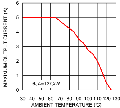
V_{IN} = 12\text{ V} , V_{OUT} = 5\text{ V}
