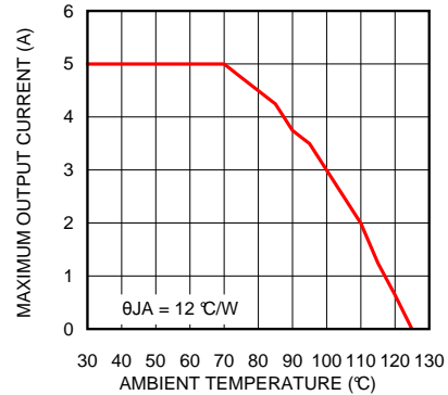
V_{IN} = 12\text{ V} , V_{OUT} = 3.3\text{ V}
