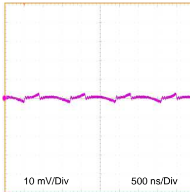
12\text{ V}_{IN} 3.3\text{ V}_O at 5\text{ A} , \text{BW} = 20\text{ MHz}
