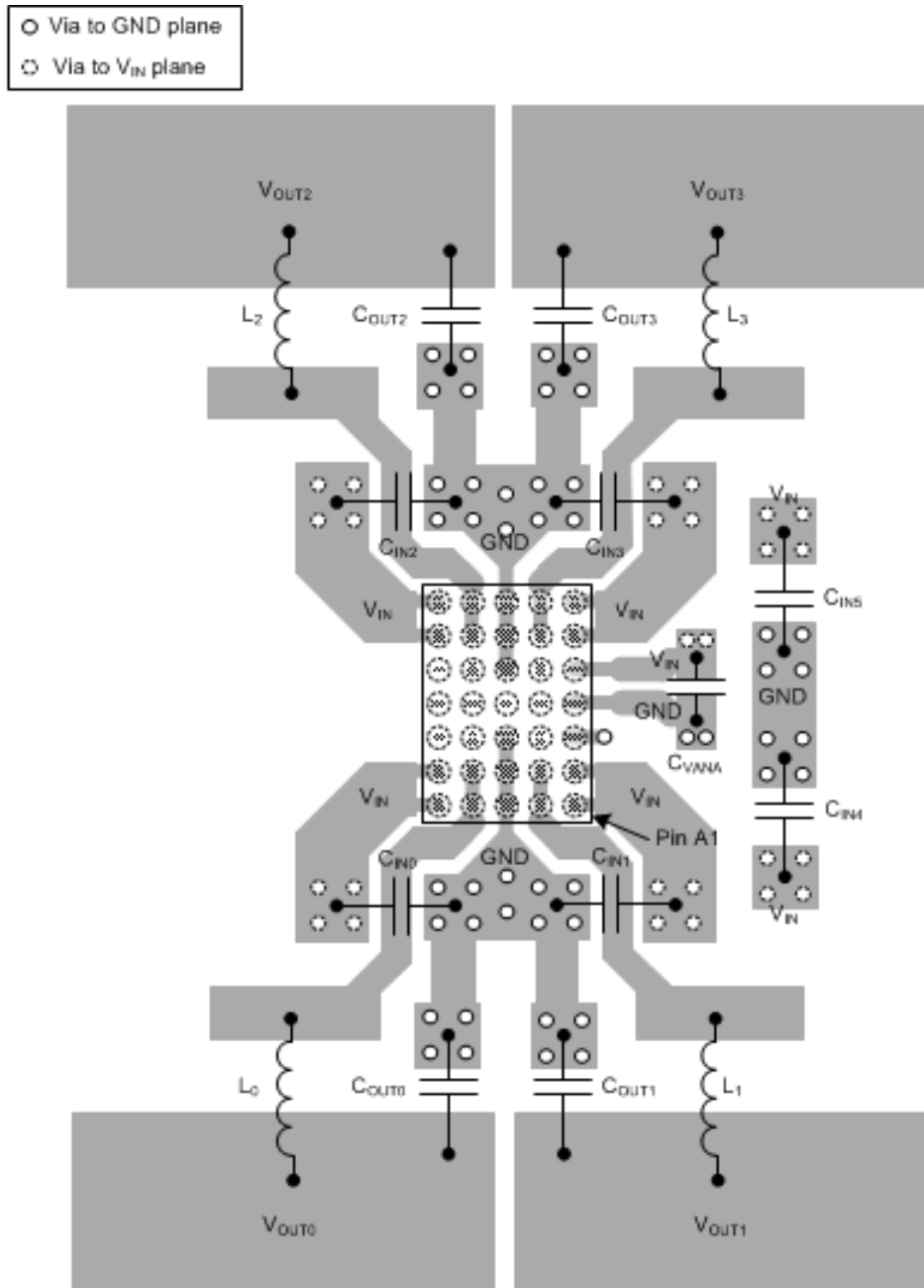
Figure 10-1. LP8758-EA Board Layout
