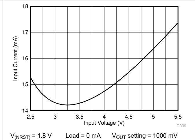
Figure 6-5. PWM Mode Current Consumption vs Input Voltage — One Output Enable
