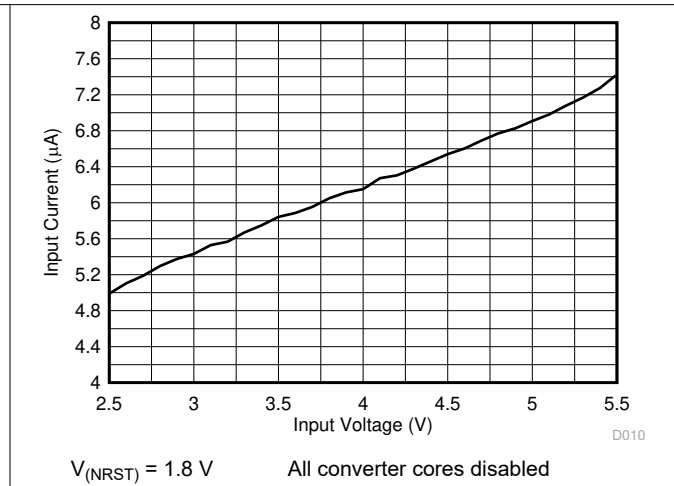
Figure 6-3. Standby Current Consumption vs Input Voltage
