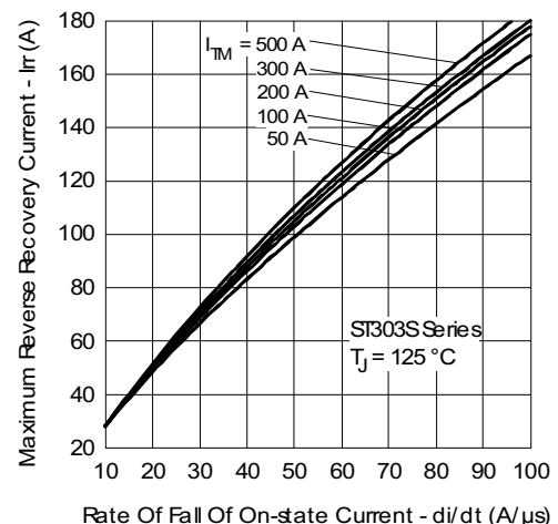
Fig. 10 - Reverse Recovery Current Characteristics
