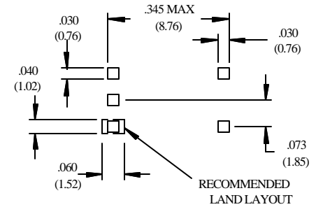
PWB FOOTPRINT
