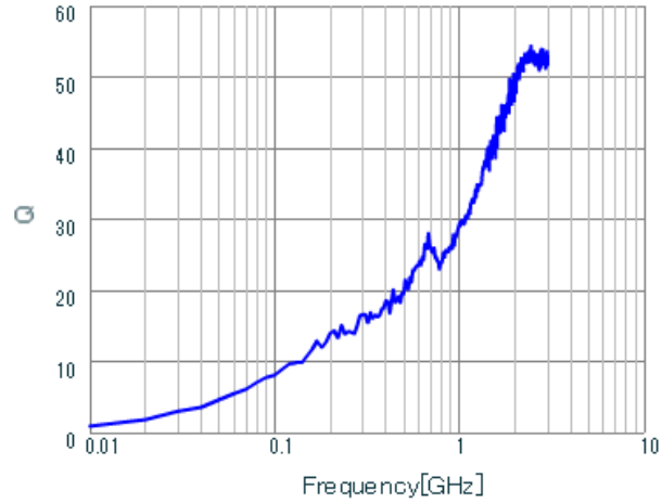
LQP02TQ0N3C02 Q.
