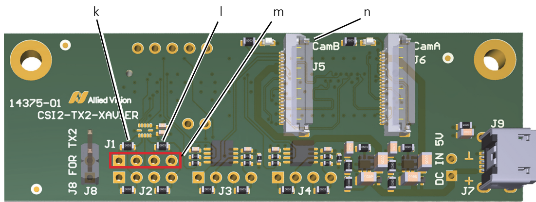
Figure 16: Desoldering resistors and soldering a pin header for Camera B
