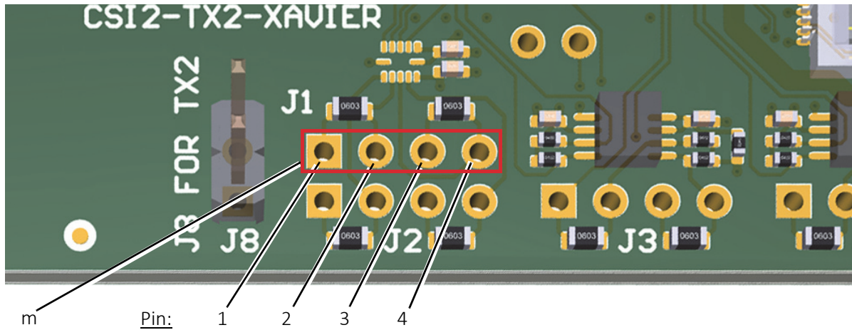
Figure 17: Connecting the I/Os for Camera B
