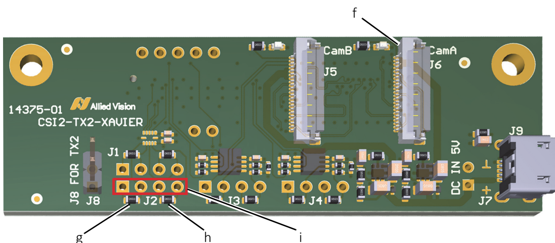
Figure 14: Desoldering resistors and soldering a pin header for Camera A
