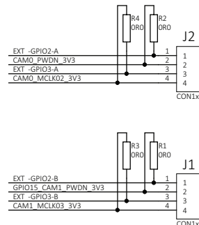
Figure 4: Adapter for Jetson TX2 and Xavier electronic schematics, part 1
