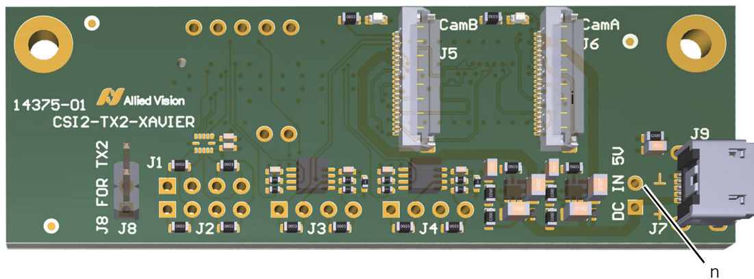
Figure 18: Connecting GND
