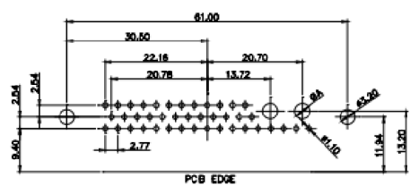
43W2 Male
