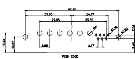
13W6 Male
