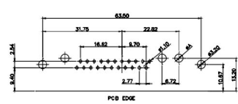
25W3 Female
