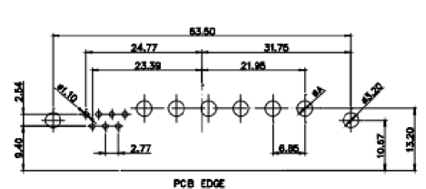
13W6 Female
