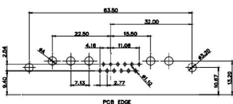
17W5 Female
