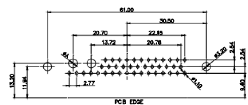
43W2 Female
