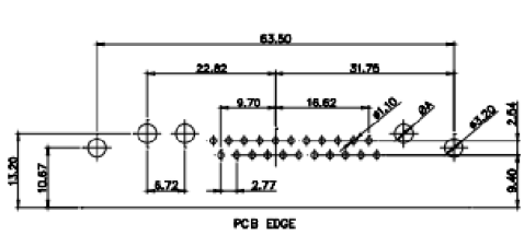
25W3 Male
