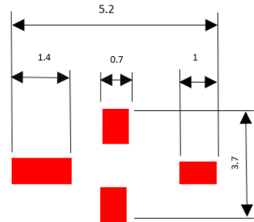
PCB Footprint
