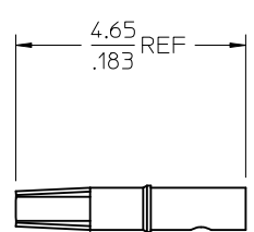
CENTER CONTACT
