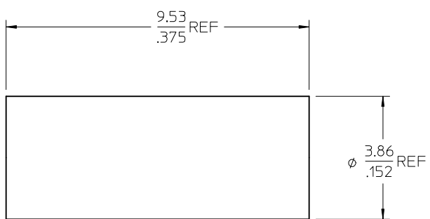
CRIMP TUBE
