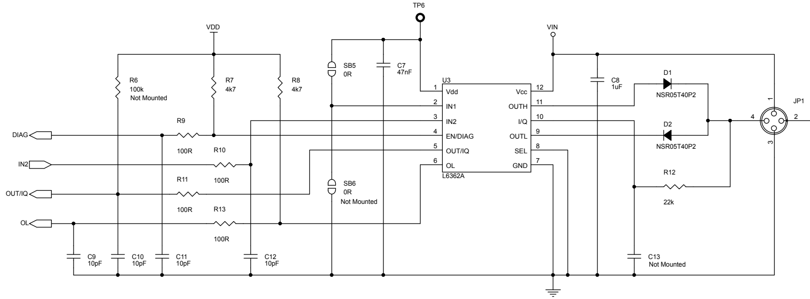
Figure 60. STEVAL-IDP005V1 schematic – IO-Link
