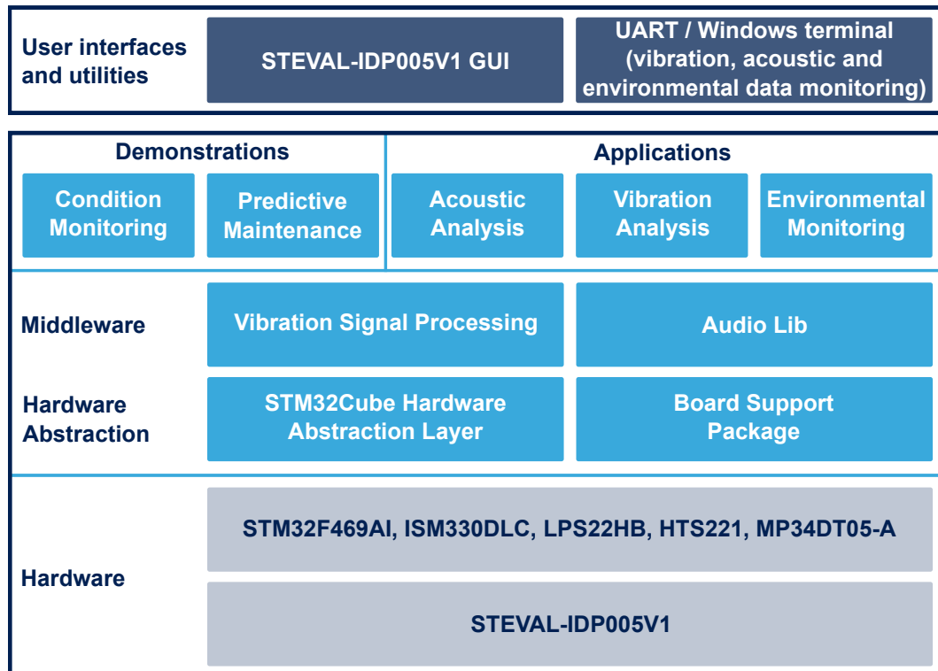
Figure 25. STSW-BFA001V1 firmware architecture
