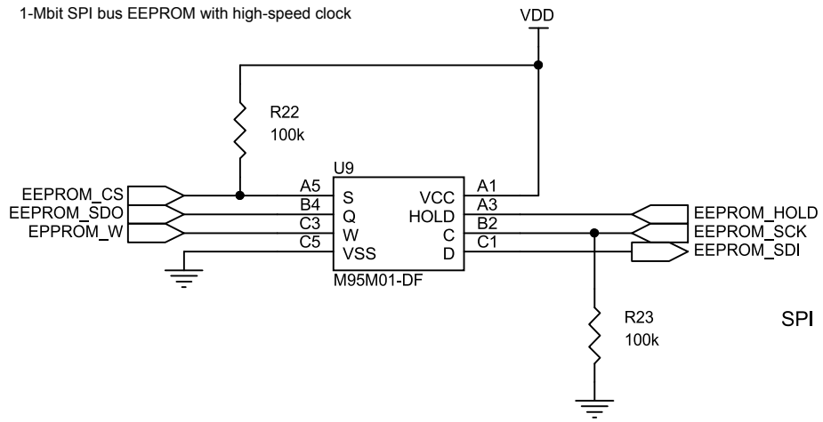
Figure 62. STEVAL-IDP005V1 schematic – EEPROM
