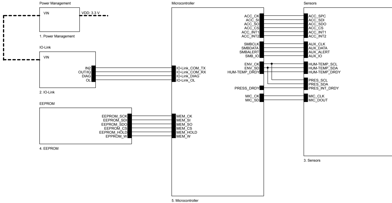
Figure 58. STEVAL-IDP005V1 schematic – General purpose industrial sensor
