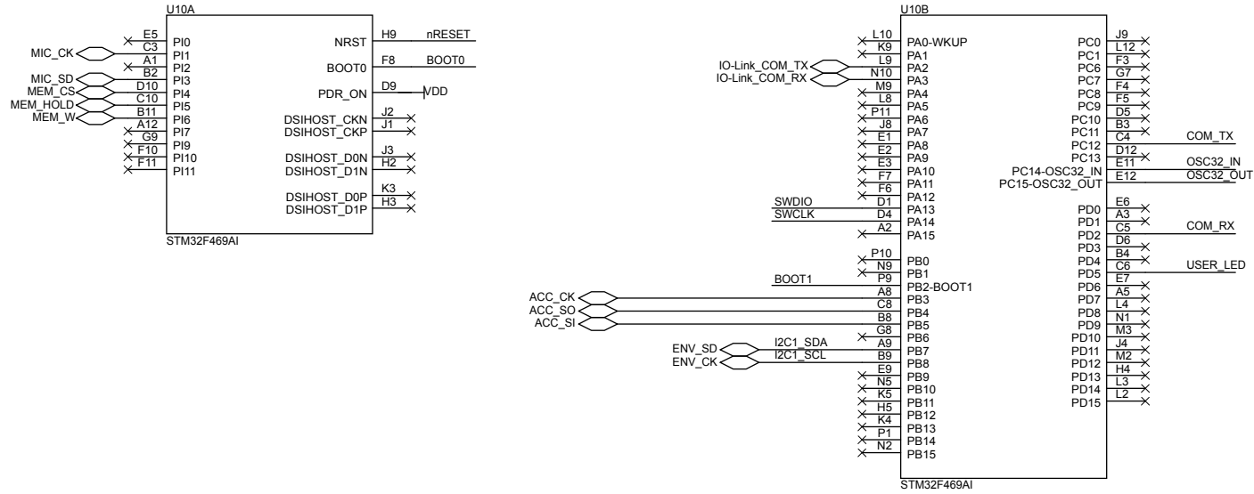
Figure 63. STEVAL-IDP005V1 schematic – Microcontroller (part A)
