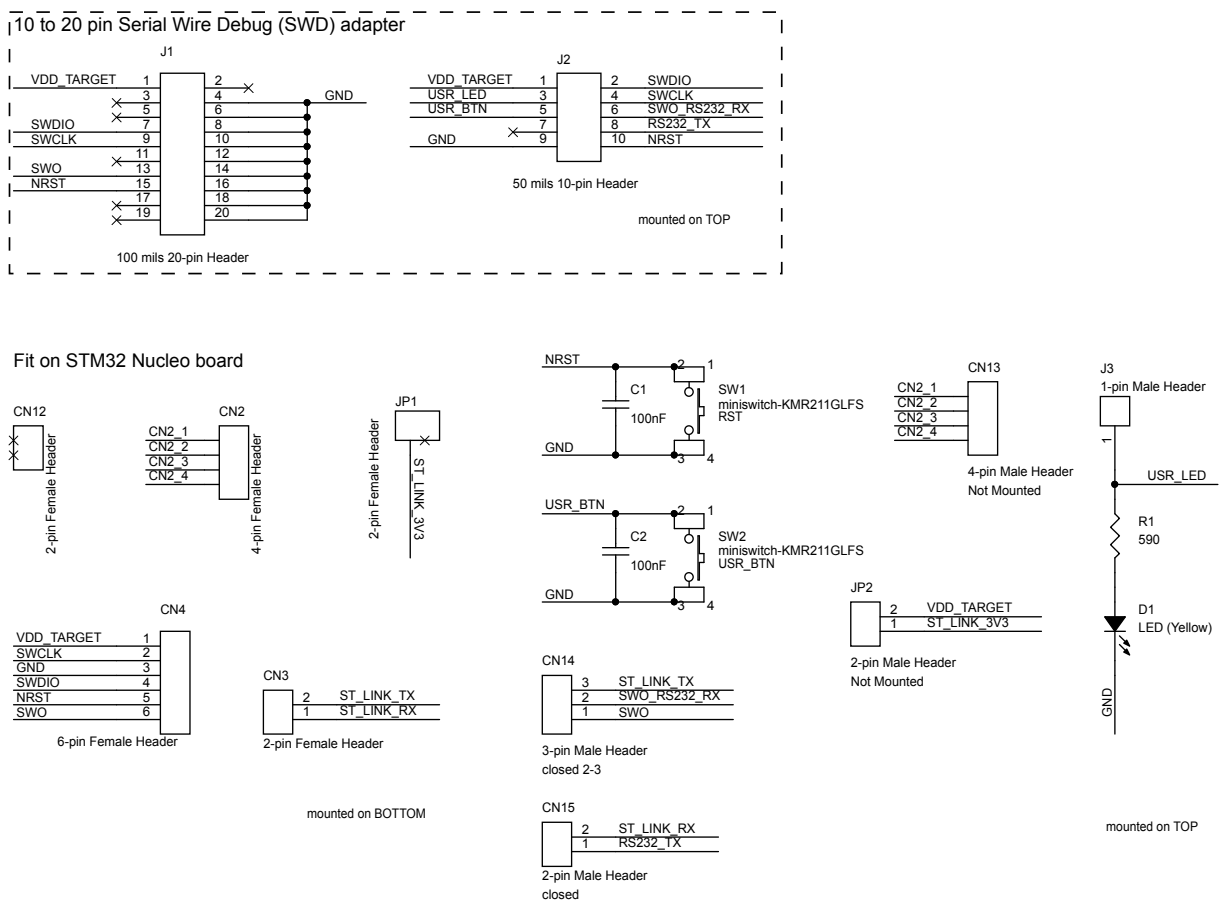
Figure 15. STEVAL-UKI001V1 schematic
