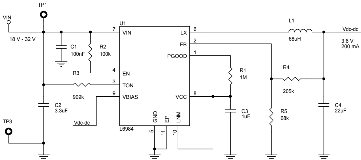
Figure 59. STEVAL-IDP005V1 schematic – Power management
