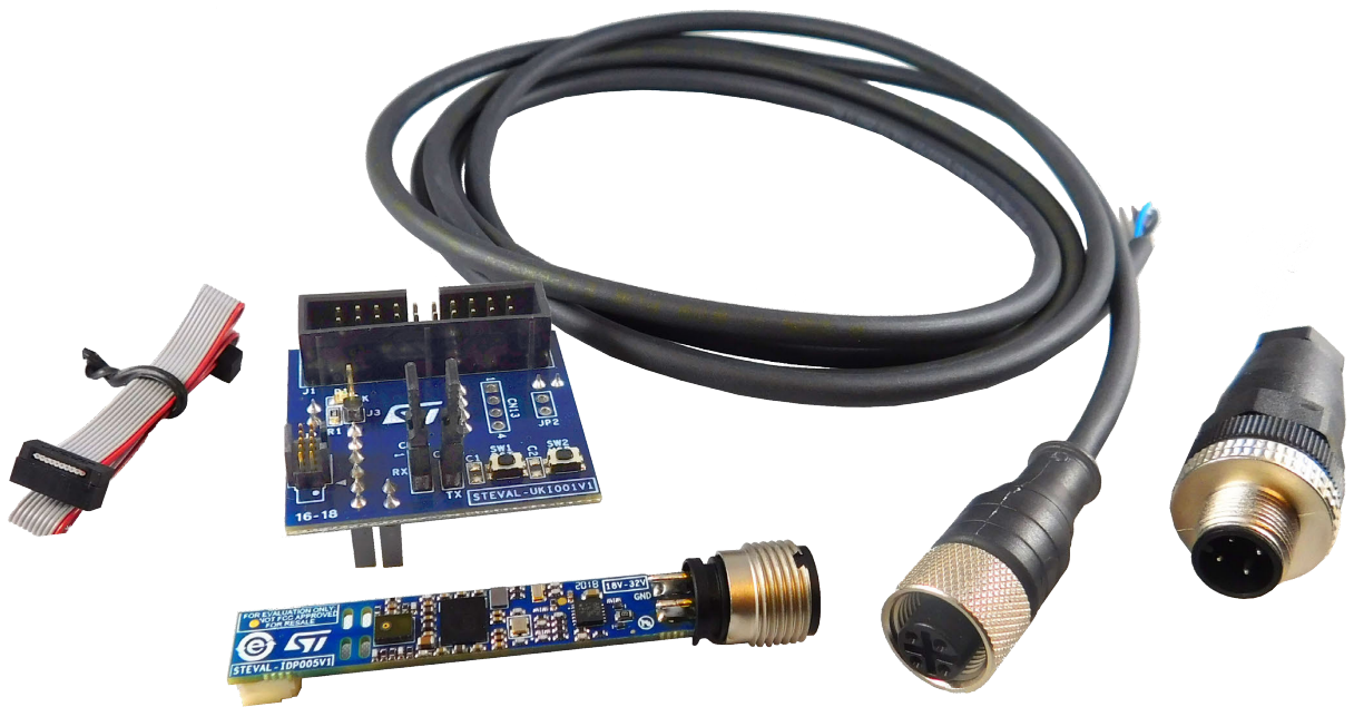
Figure 3. STEVAL-IDP005V1 board - top
