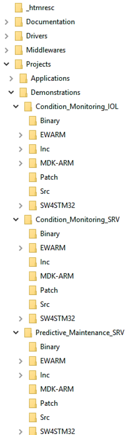
Figure 30. Demonstrations folders
