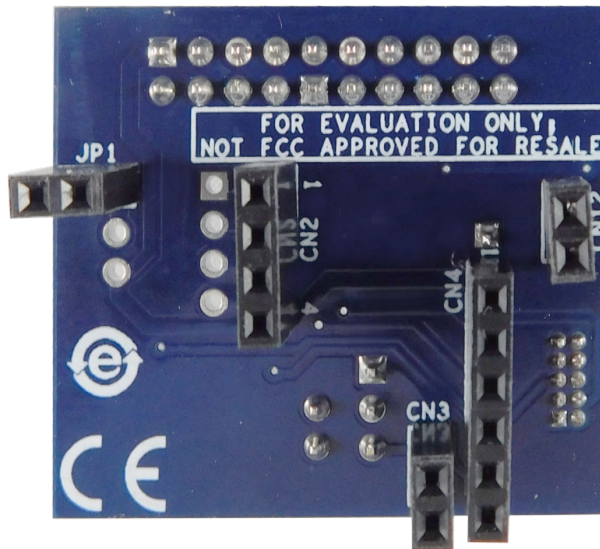
Figure 17. STEVAL-UKI001V1 bottom view
