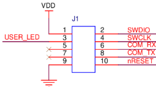
Figure 10. Enhanced SWD connector
