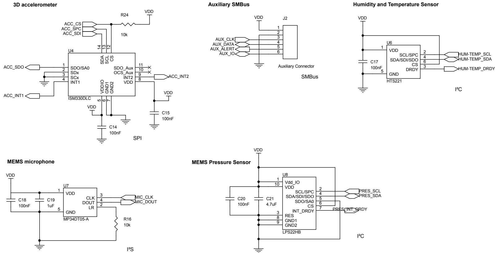
Figure 61. STEVAL-IDP005V1 schematic – Sensors
