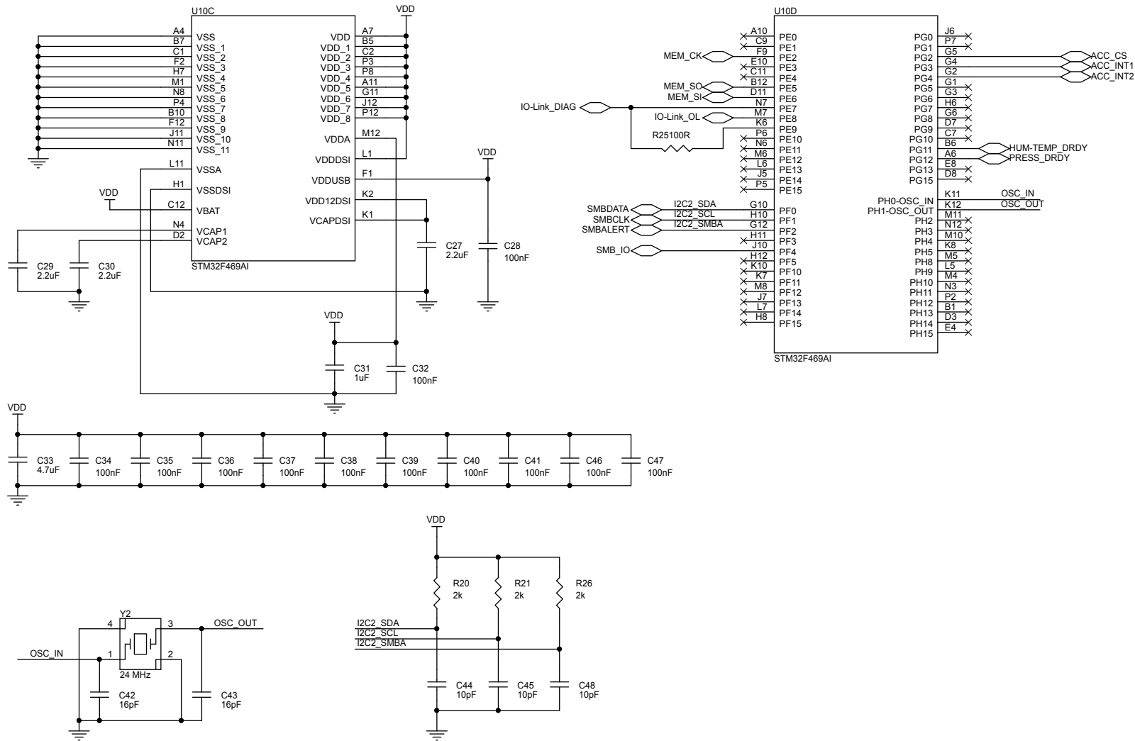
Figure 64. STEVAL-IDP005V1 schematic – Microcontroller (part B)
