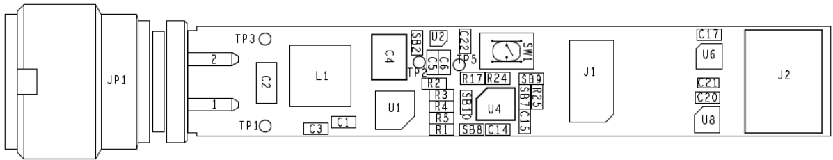
Figure 6. STEVAL-IDP005V1 bottom side components
