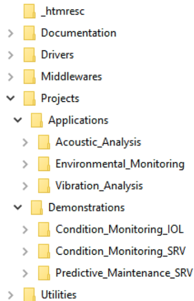
Figure 27. Projects folders
