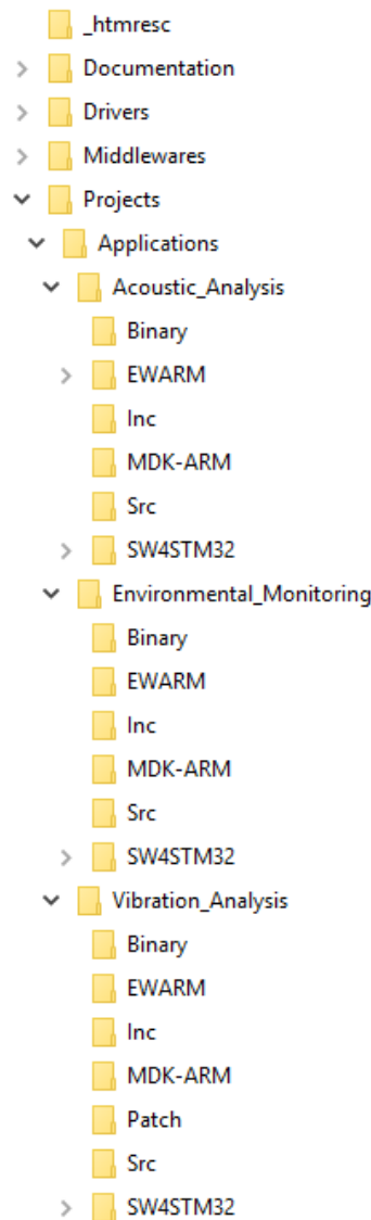
Figure 28. Applications folders
