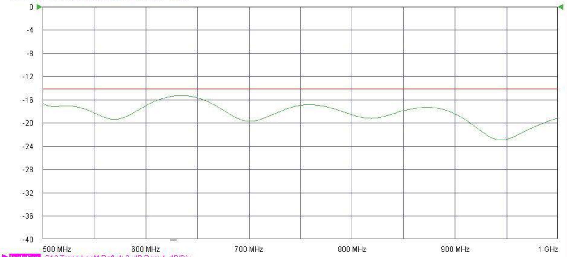
Isolation S12 Trans LogM RefLvl: 0 dB Res: 4 dB/Div
