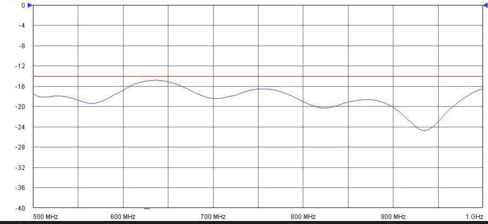
P1 VSWR S11 Refl LogM RefLvl: 0 dB Res: 4 dB/Div
