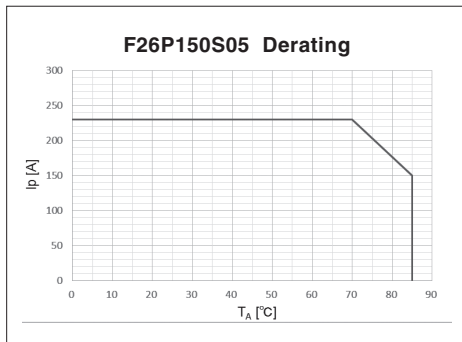
Figure 6 : Ip vs TA for F26P150S05
