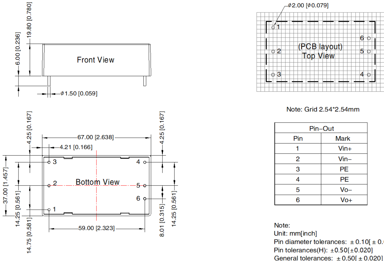
Figure 5. Mechanical drawing
