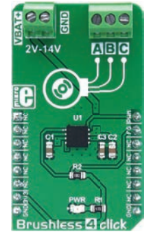
Brushless 4 Click
