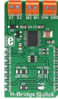
H-Bridge 2 Click
