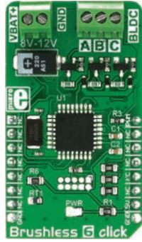
Brushless 6 Click
