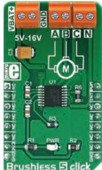
Brushless 5 Click
