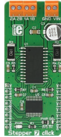
Stepper 7 Click
