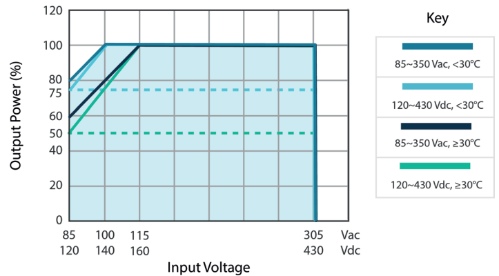
INPUT VOLTAGE DERATING CURVE 5V model [<30°C, ≥30°C]
