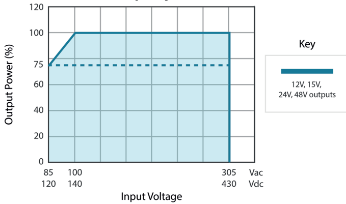
INPUT VOLTAGE DERATING CURVE 12V, 15V, 24V, 48V models [25°C]
