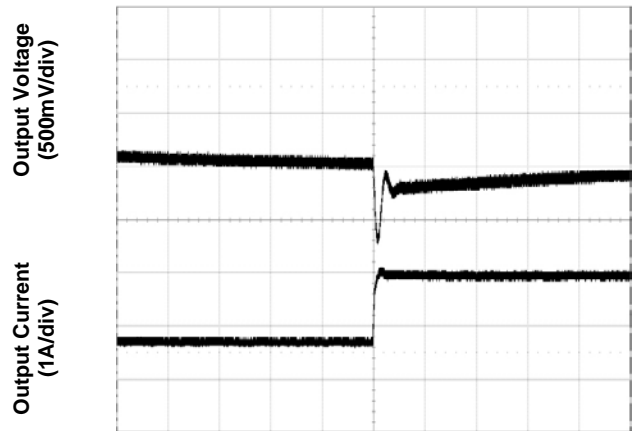
Figure 8. Transient Load Response (typical V_{in} , load current steps from 50% to 75% at a slew rate 0.1A/\mu s )
