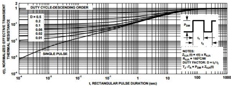
Figure 12. Junction-to-Ambient Transient Thermal Response Curve
