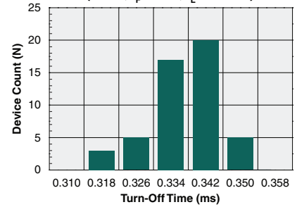
Typical Turn-Off Time (N=50, I_F=5mA, I_L=150mA )
