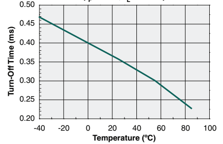
Typical Turn-Off Time vs. Temperature ( I_F=5mA, I_L=80mA )
