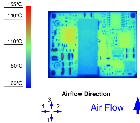
Figure 8. Thermal Image for Airflow Direction 3 (6A output, 55°C ambient, nature convection, typical Vin, open frame, unit soldered onto a fixture board)
