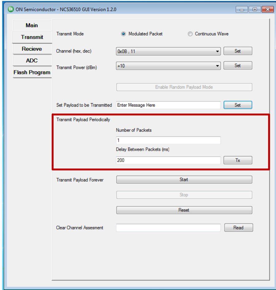
Figure 7. GUI-Transmit-Periodically
