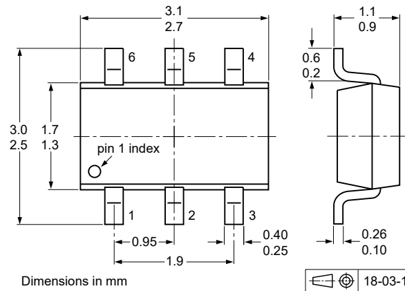
Fig. 8. Package outline SC-74; TSOP6 (SOT457)
