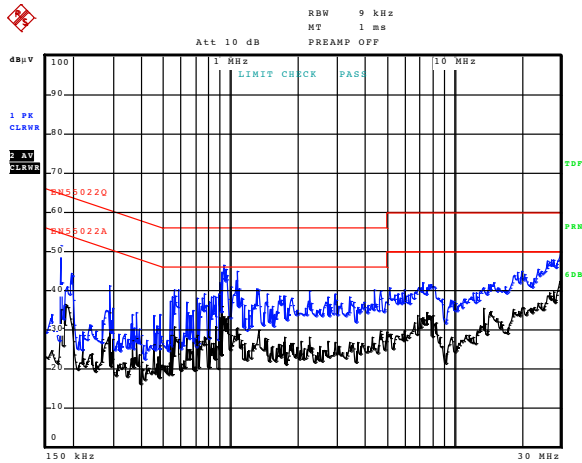
Figure 35. Conducted EMI, 115 Vac, LINE
