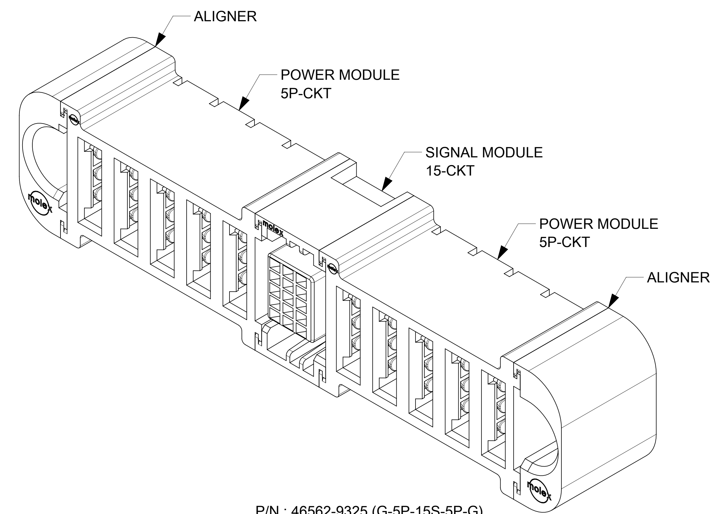
P/N : 46562-9325 (G-5P-15S-5P-G)
