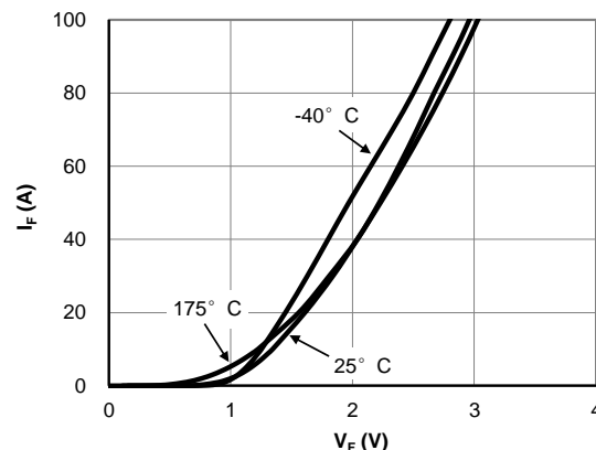
Figure 4: Diode Characteristic
