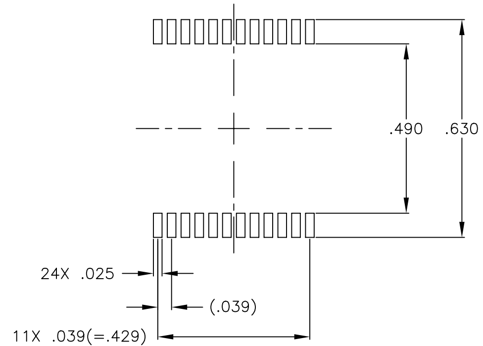
SUGGESTED LAND PATTERN
