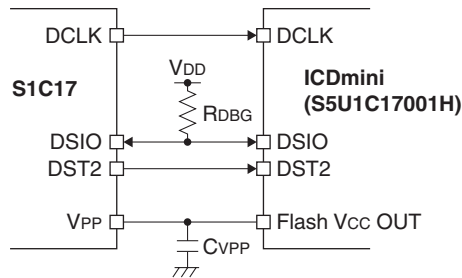
Figure 4.3.3.1 External Connection
