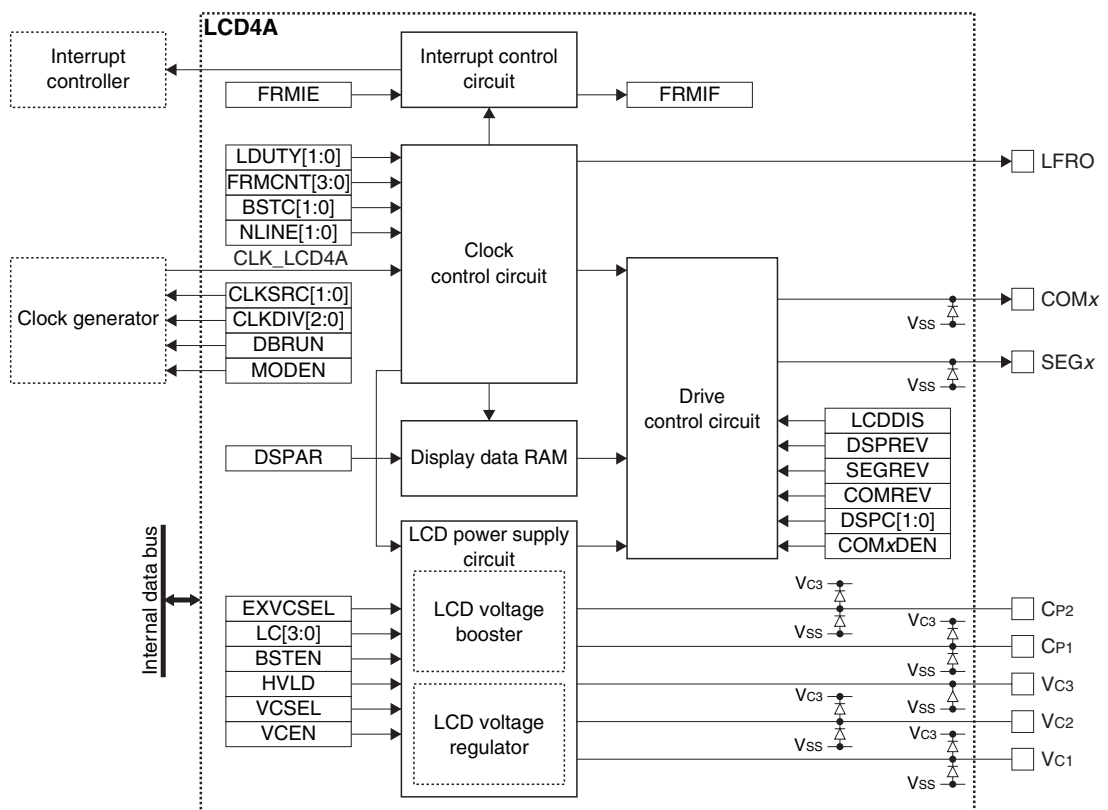
Figure 18.1.1 LCD4A Configuration
