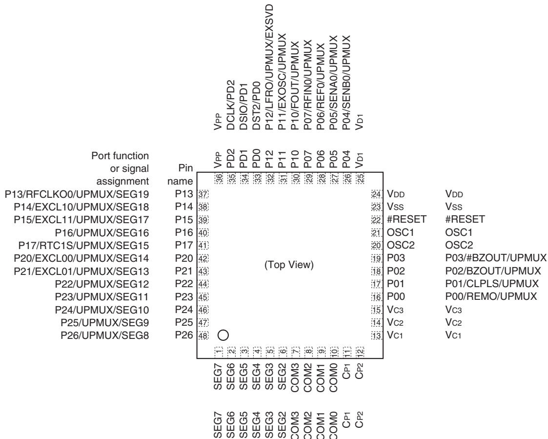
Figure 1.3.1.3 S1C17W13 Pin Configuration Diagram (SQFN7-48PIN)
