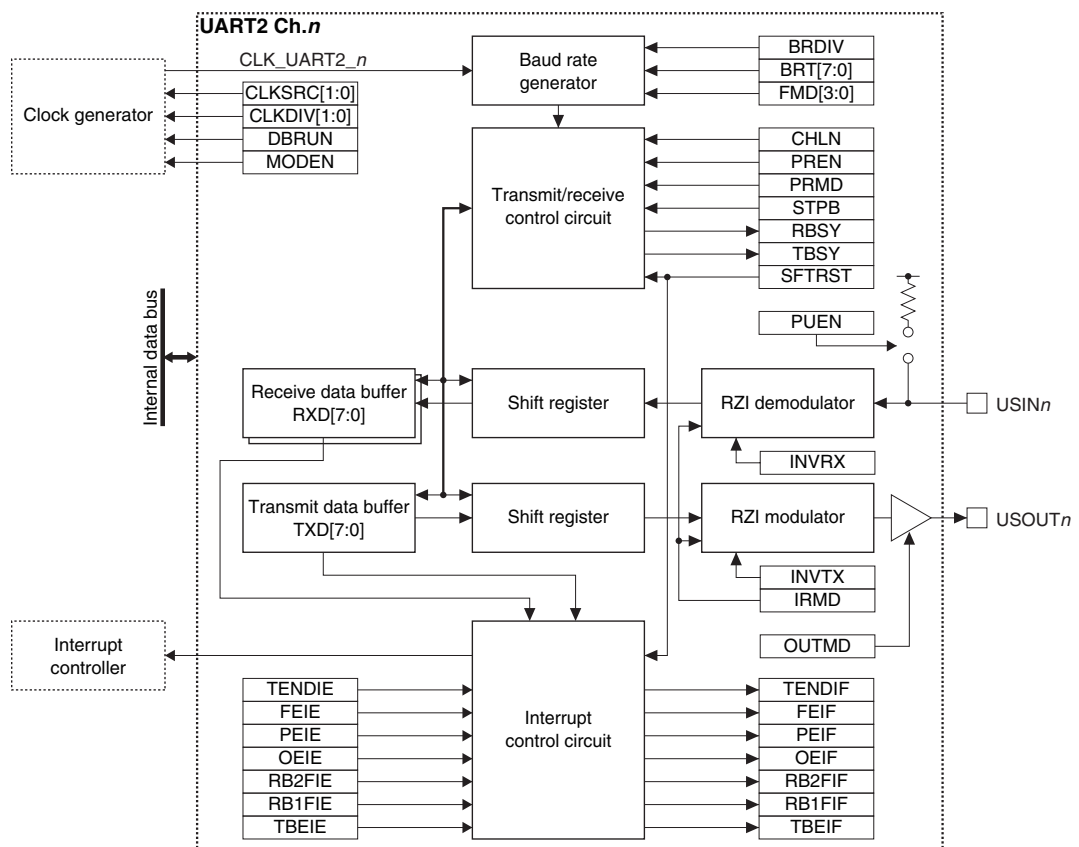
Figure 12.1.1 UART2 Configuration
