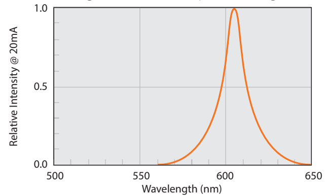
Fig. 6 Direct Radiation
