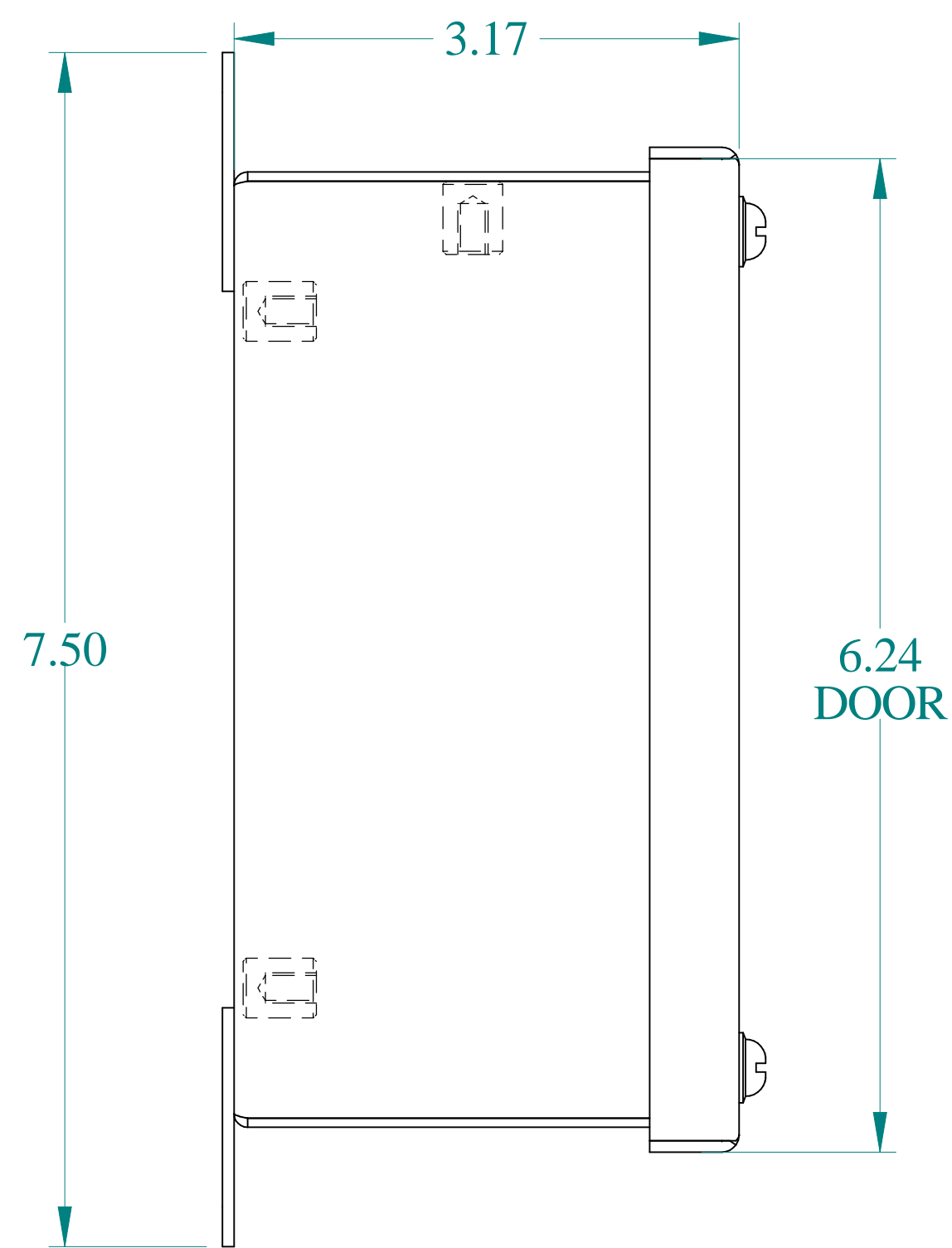
SIDE VIEW
