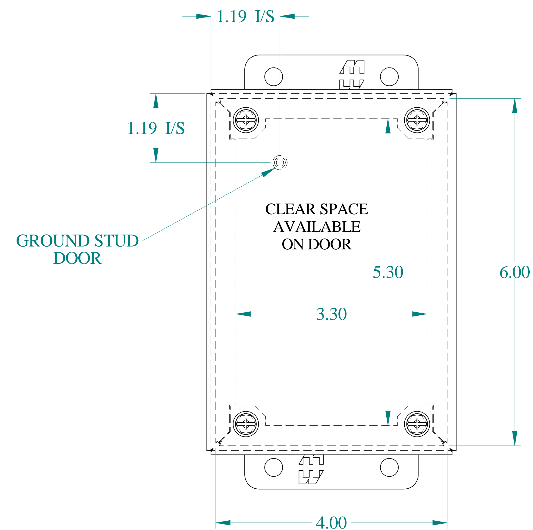
FRONT VIEW
