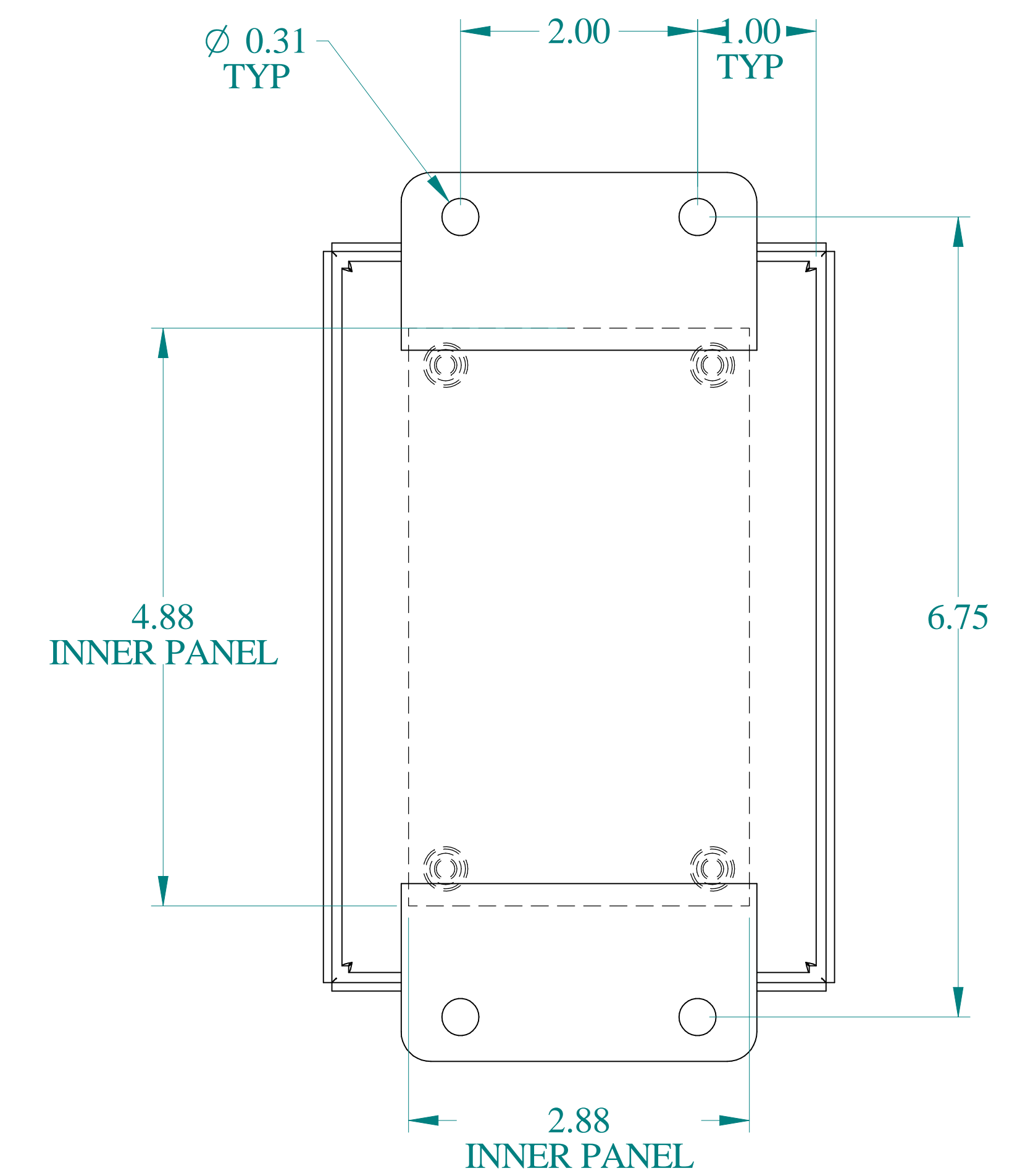
BACK VIEW
