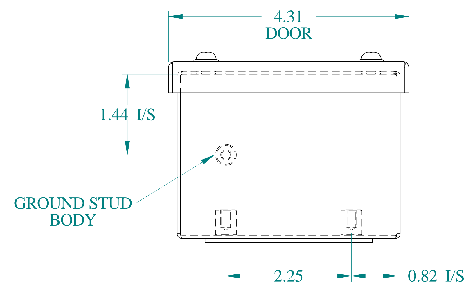
BOTTOM VIEW
