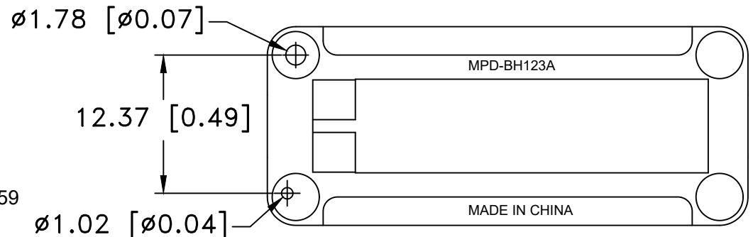
BOTTOM VIEW
