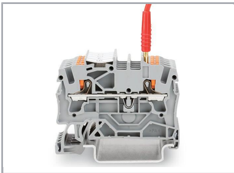
Testing with a 2 mm \varnothing test plug (max. 42 V).
